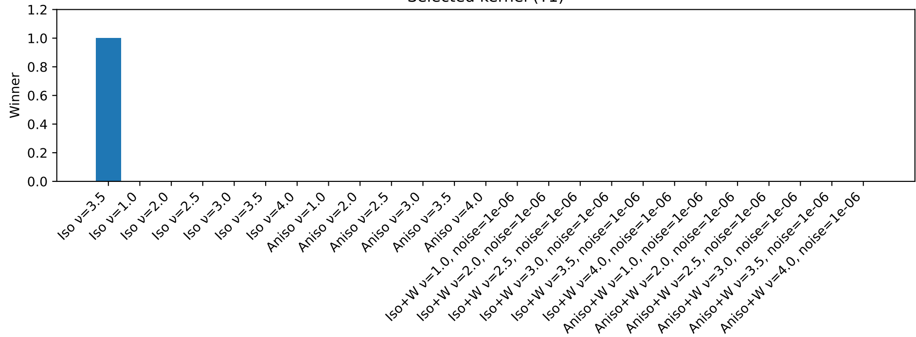
Selected kernel (T1)
