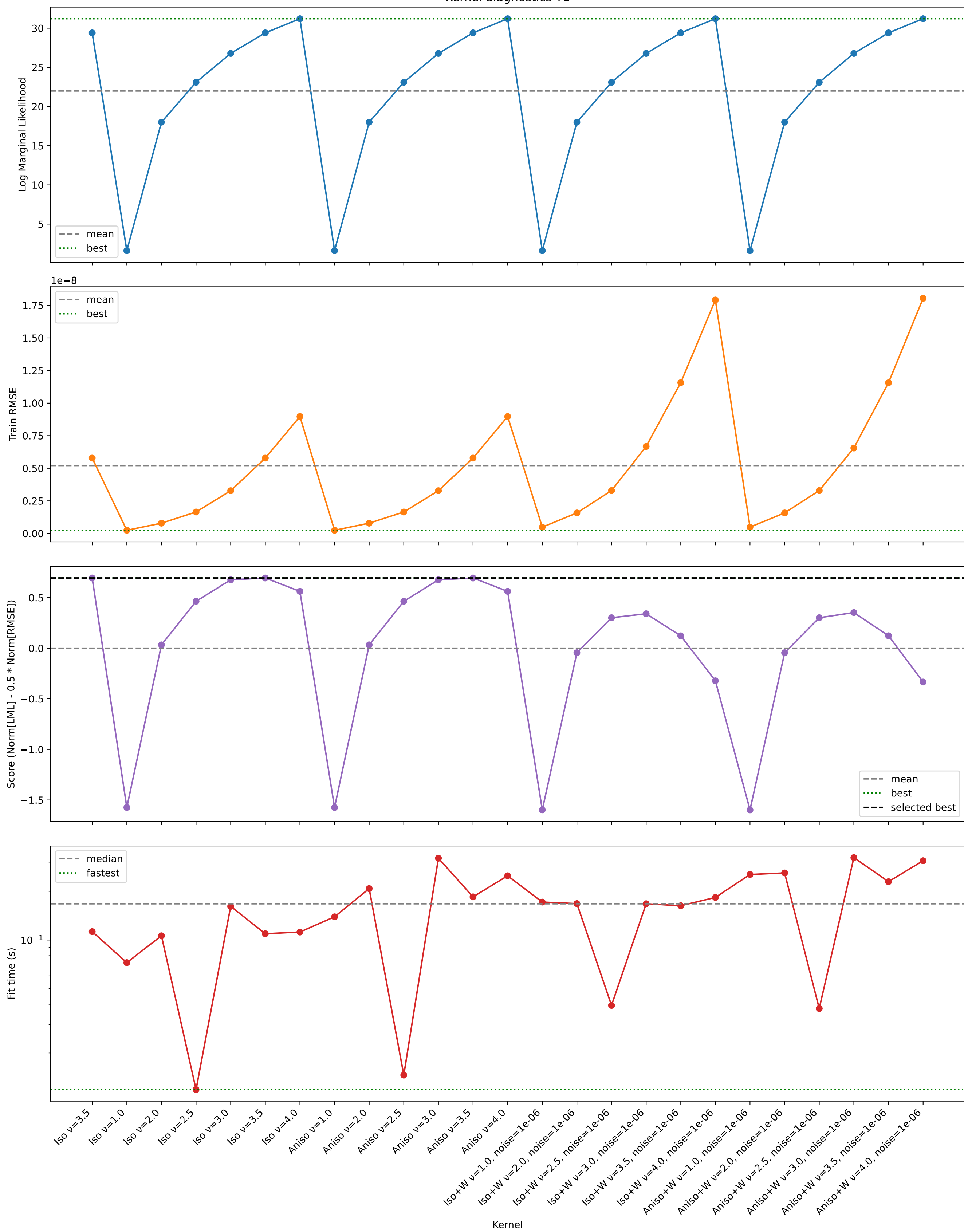
Kernel diagnostics T1
