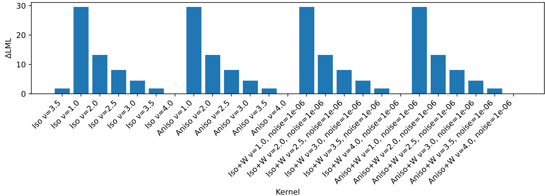
Difference from best LML (T1)
